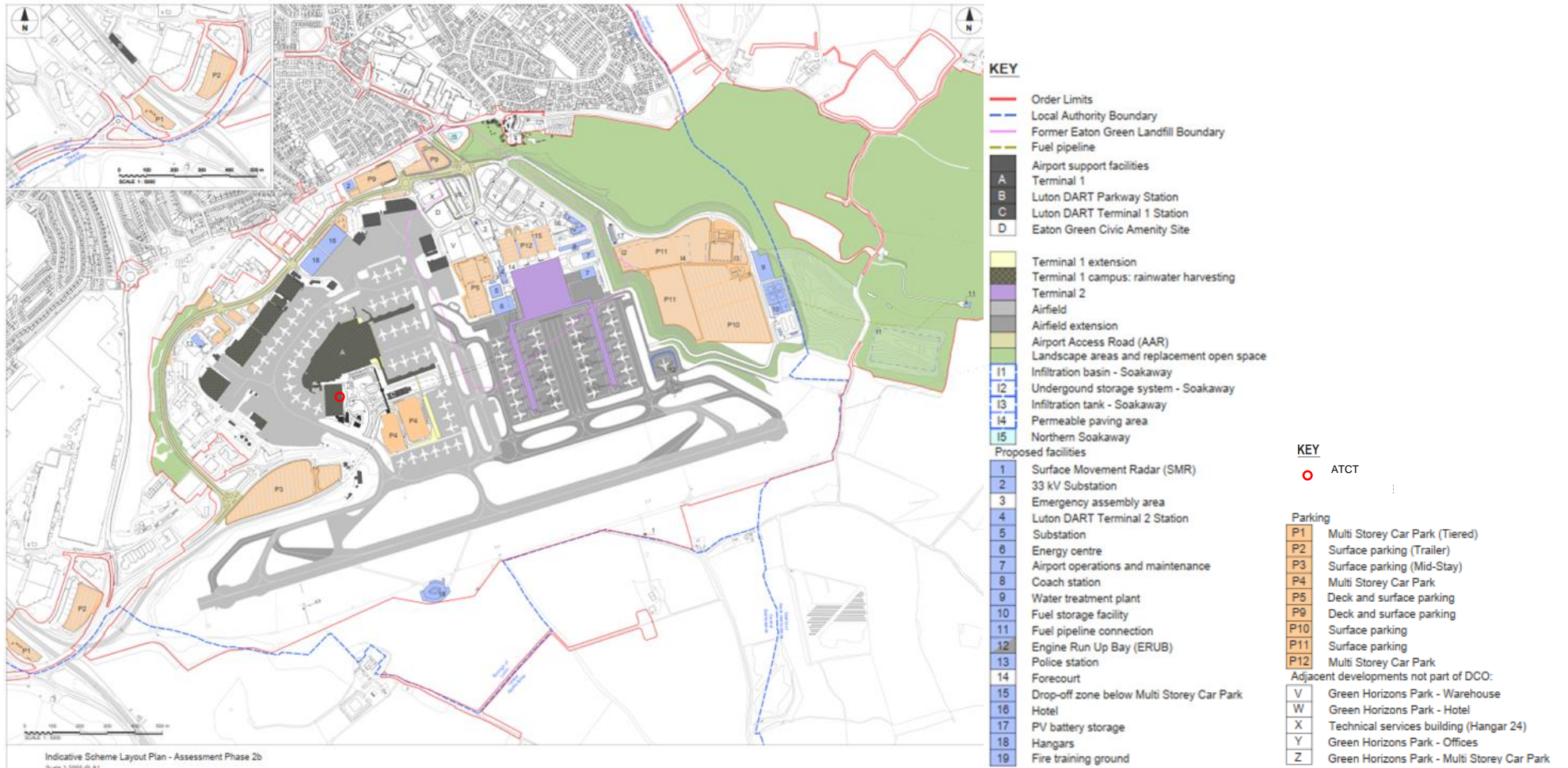
Figure 4-3 Proposed Site Layout (replica of 4.02 Scheme Layout Plans [TR020001/APP/4.02AS-010])
